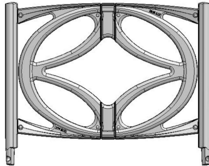
INTERLAKEN 2'x 2' PLANTER FENCE scale 1:10
