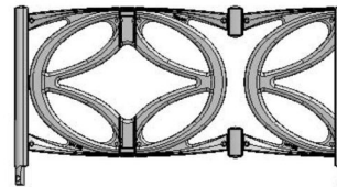
INTERLAKEN 3'x 6' PLANTER FENCE scale 1:20
