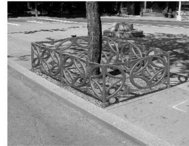
INTERLAKEN 3'x 6' PLANTER FENCE scale 1:20
