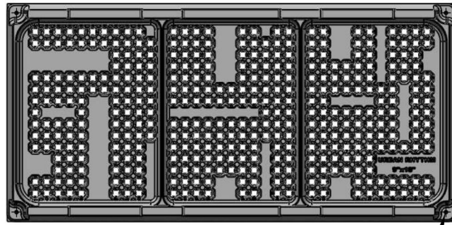
REAR scale 1:5
